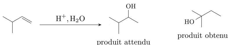
FIGURE 10.2 – Illustration de transposition
